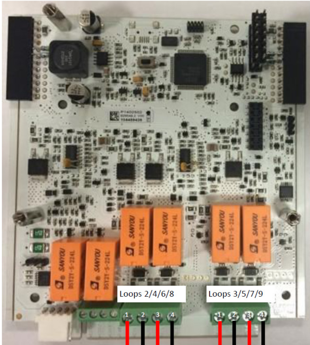
Connector J9
